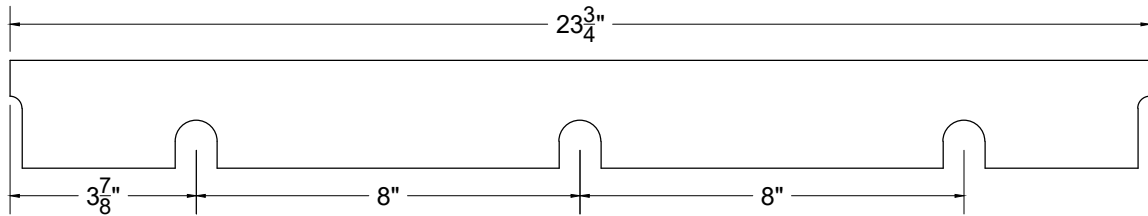
FRONT VIEW
